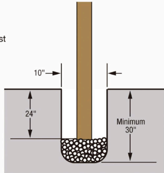
Fig 2. Setting Posts
